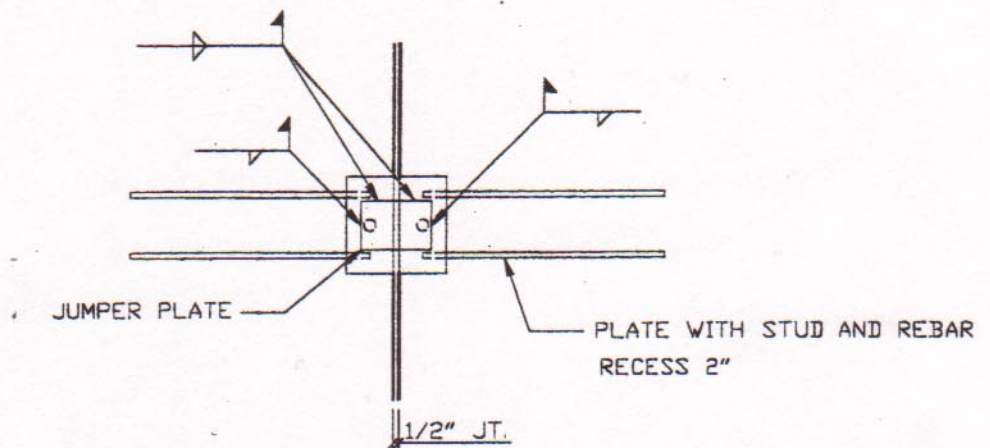
ELEVATION VIEW
