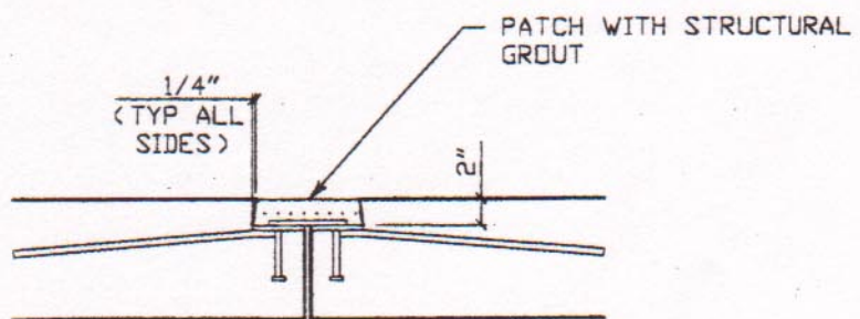
SECTION VIEW
